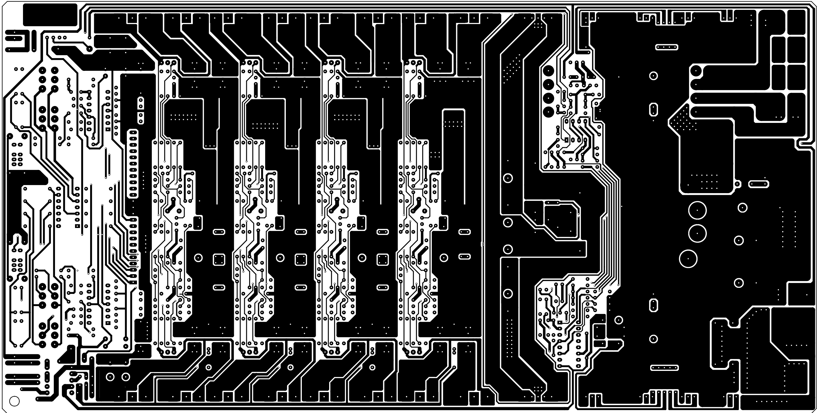
PH2200W/4—Toplayer
