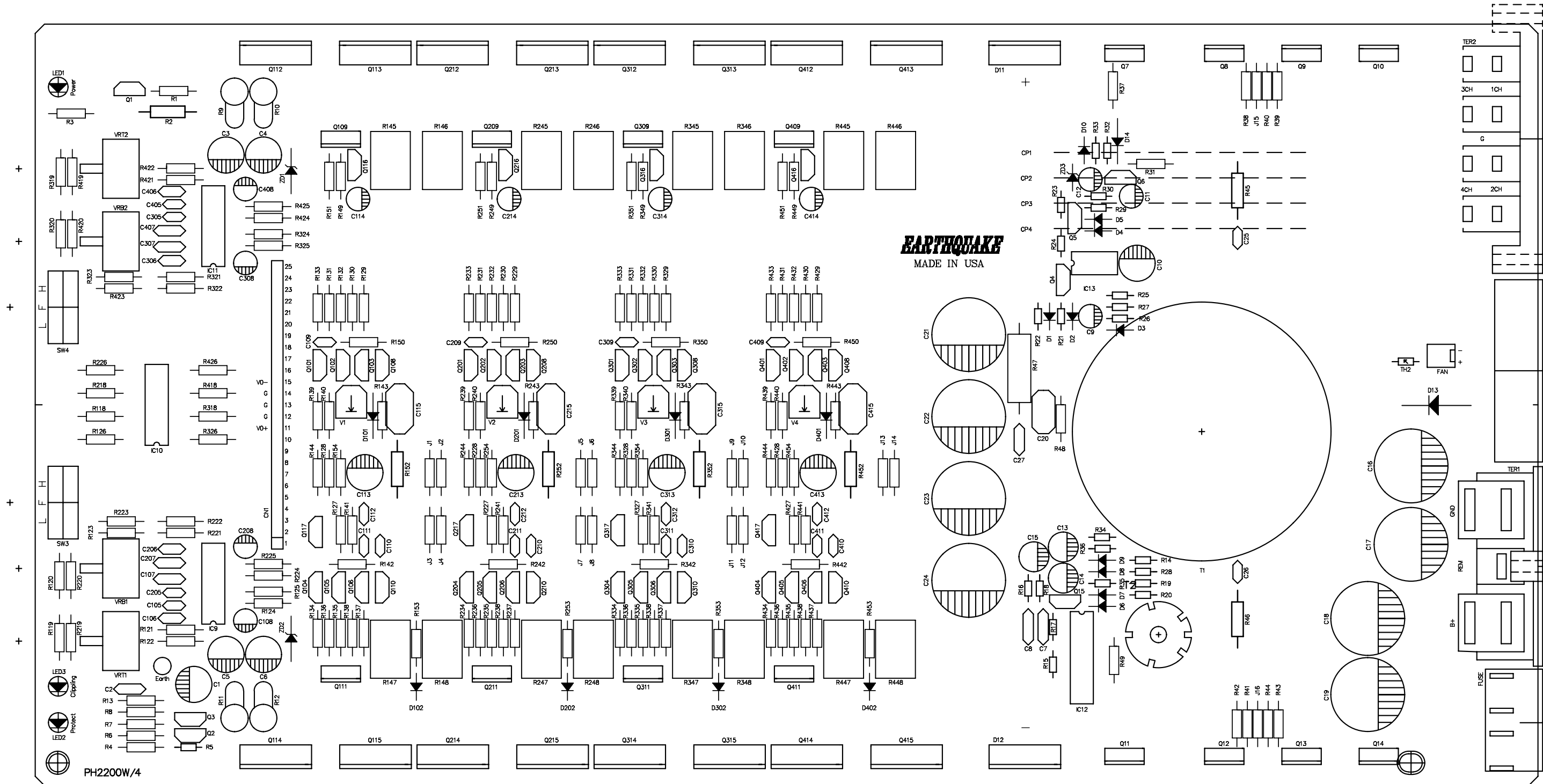
PH2200W/4—Top Overlay
