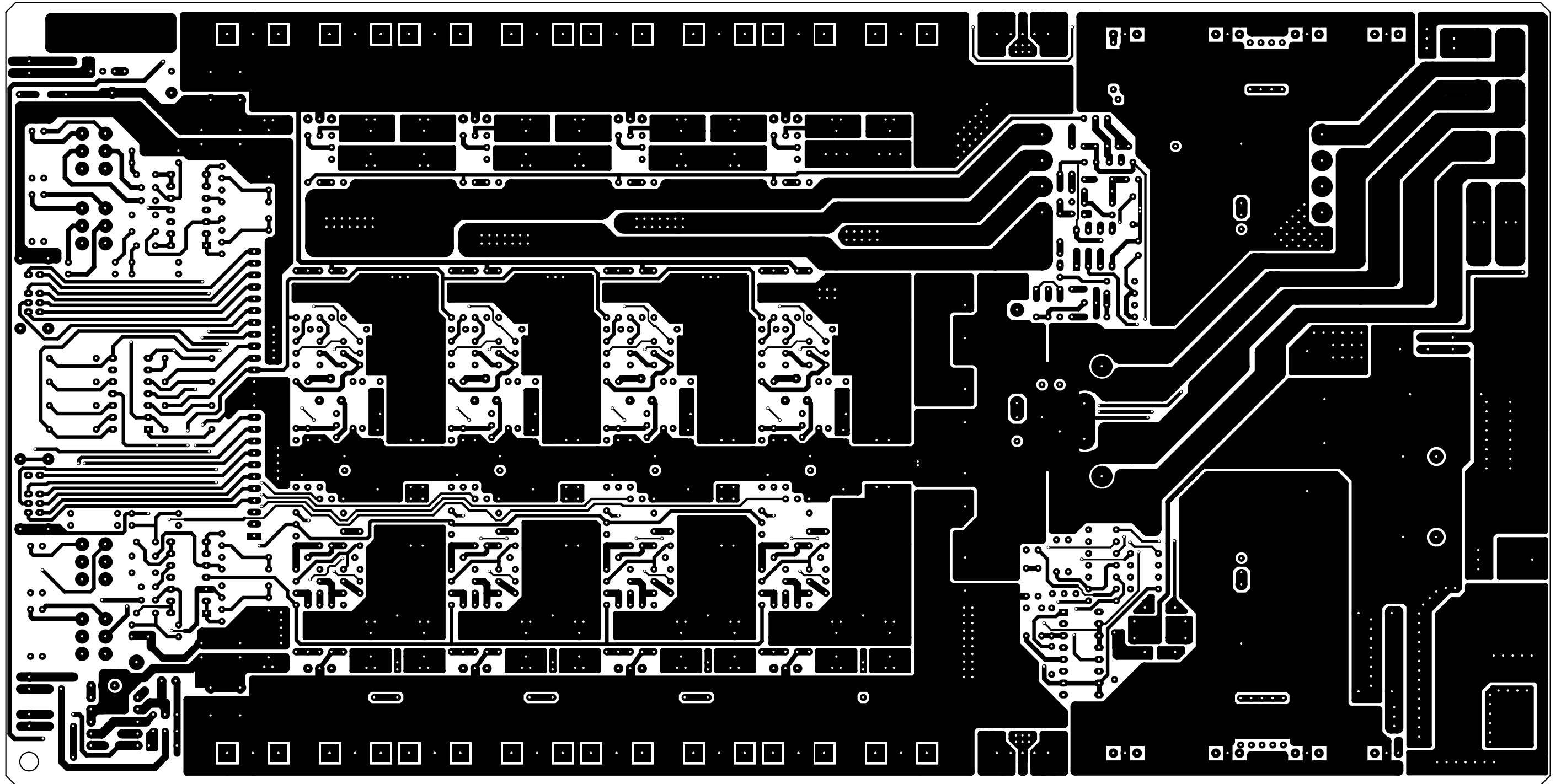
PH2200W/4-Bottomlayer
